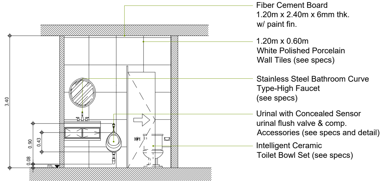
(COMMON C.R.) C SECTION - ELEVATION "B" A-08 SCALE 1:50M
