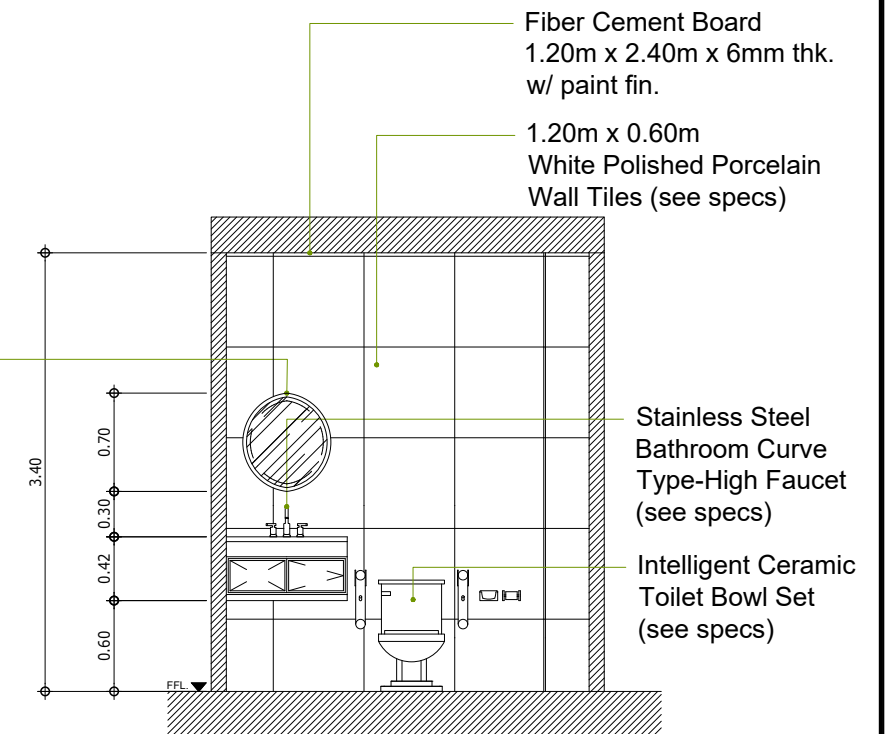
E (T&B - UNIT 101 & ROOM 101) A-07 SECTION - ELEVATION "D" SCALE 1:50M
