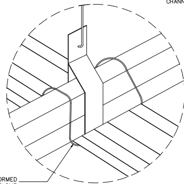
SPOT DETAIL
