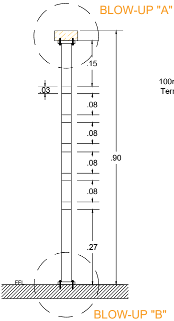
F STEEL RAILING DETAILS SCALE NTS.
