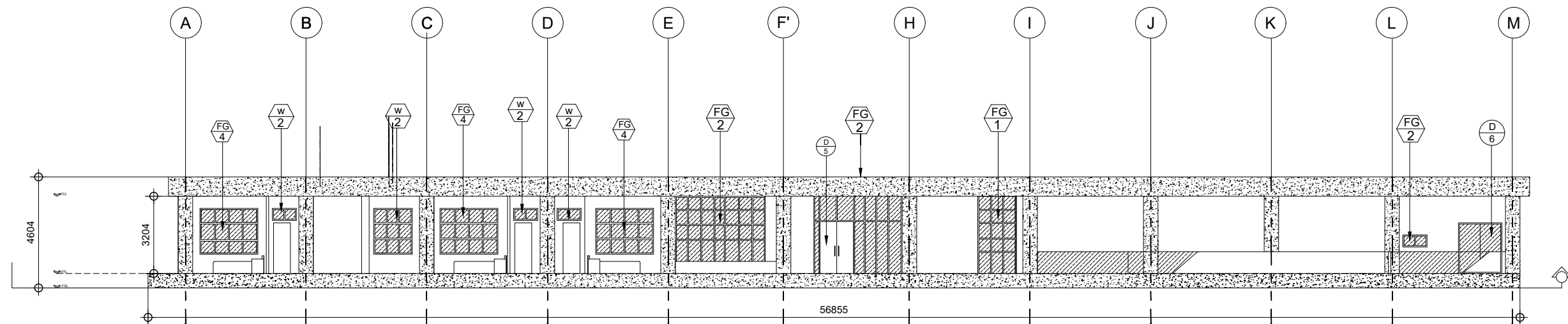
D A-04 GROUND FLOOR LONGITUDINAL SECTION SCALE 1:200M
