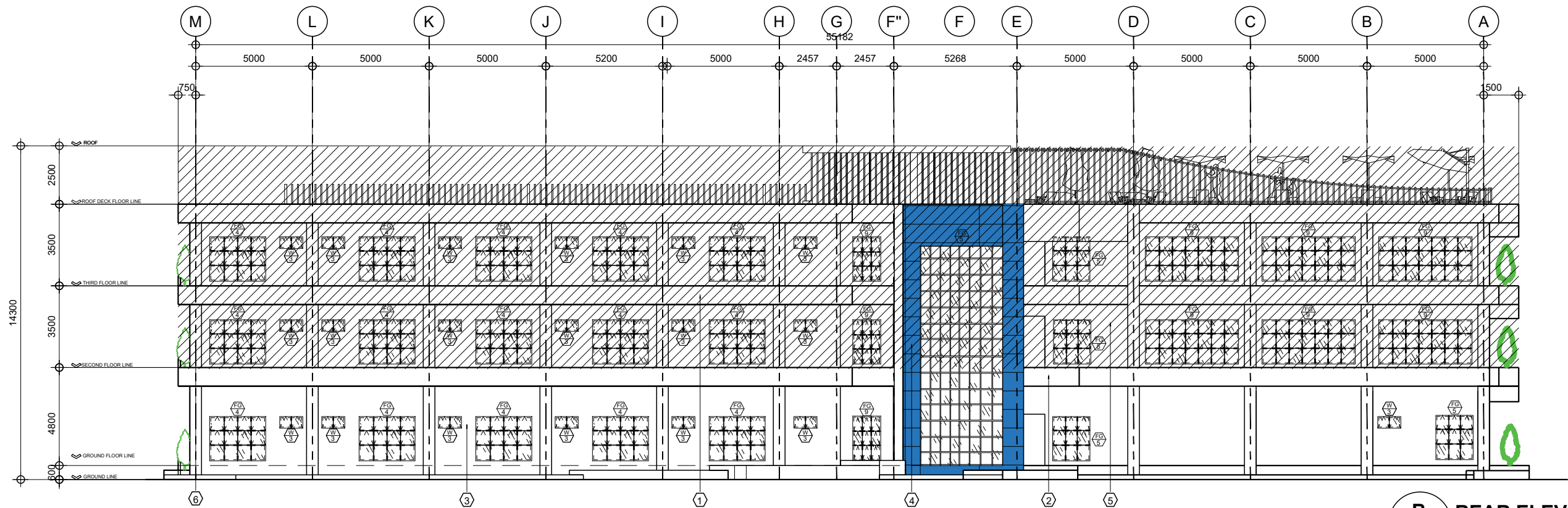
B REAR ELEVATION A-03 SCALE 1:200M
