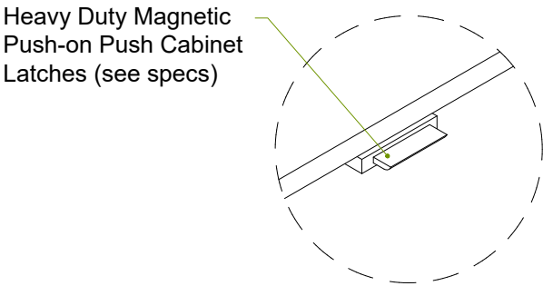
D BLOW-UP DETAIL "C" SCALE NTS.
