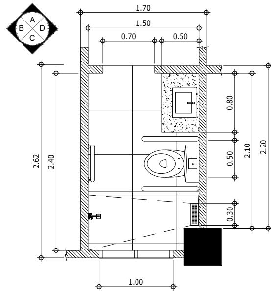
PLAN A (T&B - UNIT 101 & ROOM 101) A-07 SCALE 1:50M
