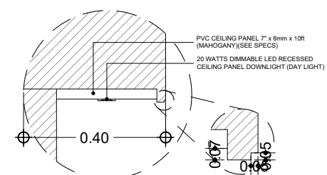
BLOW - UP DETAIL "A"
