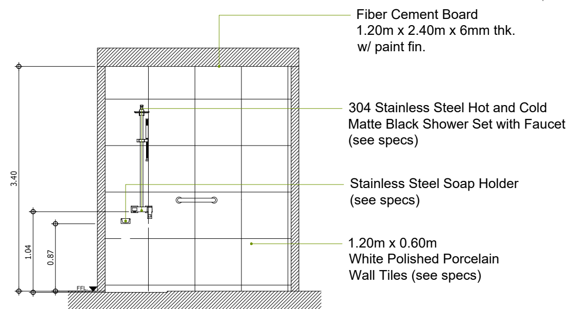
E (T&B - UNIT 101 & ROOM 101) A-07 SECTION - ELEVATION "D" SCALE 1:50M
