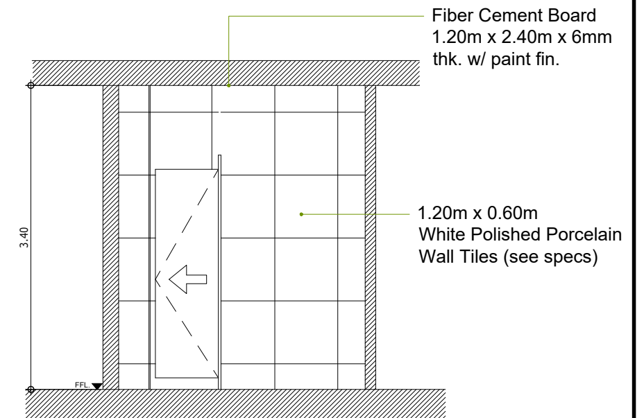
(COMMON C.R.) E SECTION - ELEVATION "D" A-08 SCALE 1:50M
