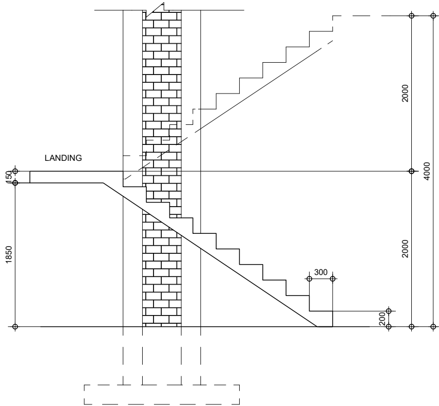
B GROUND FLOOR LEVEL STAIRS A-05 SCALE 1:50M
