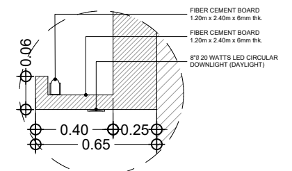
BLOW - UP DETAIL "E"
