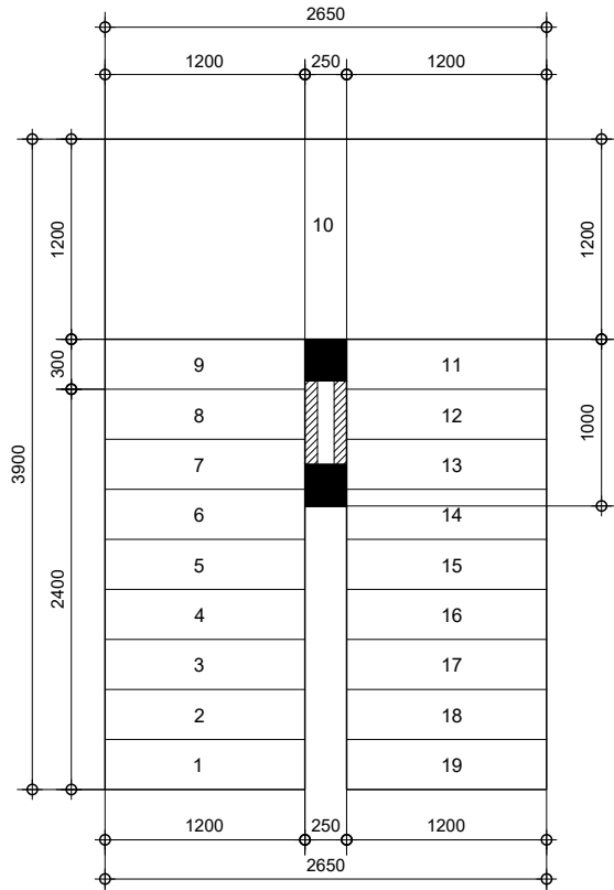
B GROUND FLOOR LEVEL STAIRS A-05 SCALE 1:50M
