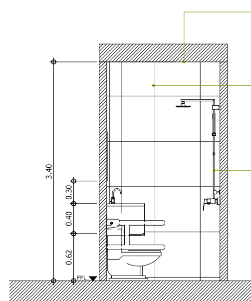
(T&B - UNIT 101 & ROOM 101) D SECTION - ELEVATION "C" A-07 SCALE 1:50M
