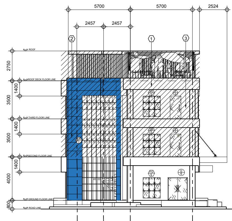
A LEFT ELEVATION
