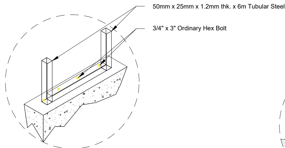
B A-13 SCALE NTS. SUNBREAKER BLOW-UP DETAIL "B"
