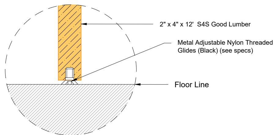
F A-13 SCALE NTS. WOODEN SLAT BLOW-UP DETAIL "B"
