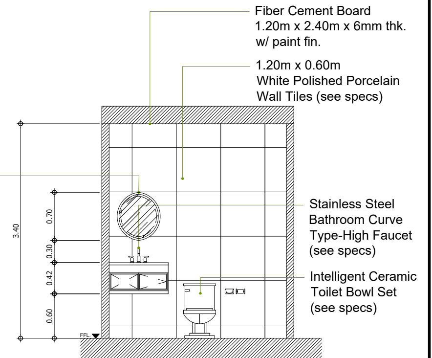
(T&B - UNIT 101 & ROOM 101) E SECTION - ELEVATION "D" A-07 SCALE 1:50M
