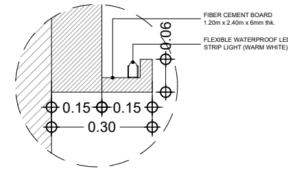
BLOW - UP DETAIL "B"
