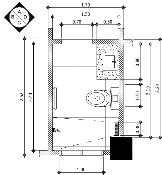
PLAN A (T&B - ROOMS & UNIT 102-103) A-09 SCALE 1:50M
