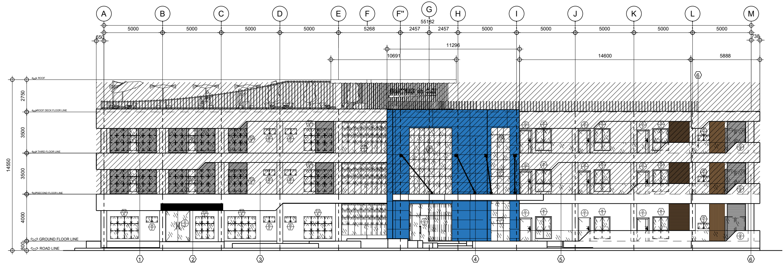
A FRONT ELEVATION A-03 SCALE 1:200M
