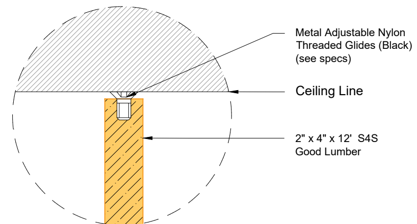
E A-13 SCALE NTS. WOODEN SLAT BLOW-UP DETAIL "A"
