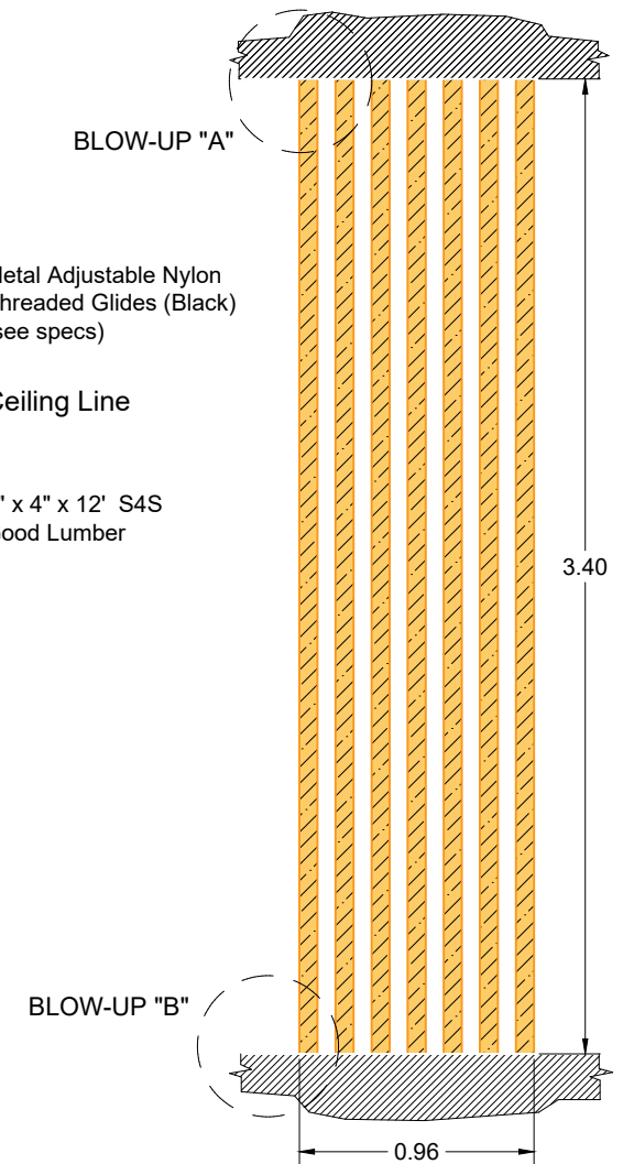
D A-13 SCALE NTS. WOODEN SLAT DETAIL
