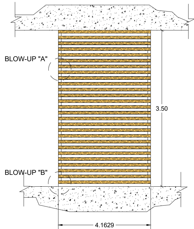
A A-13 SCALE NTS. SUNBREAKER DETAIL
