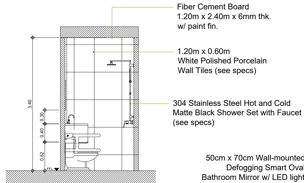
D (T&B - UNIT 101 & ROOM 101) A-07 SECTION - ELEVATION "C" SCALE 1:50M
