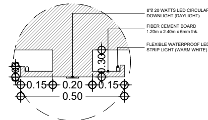
BLOW - UP DETAIL "C"
