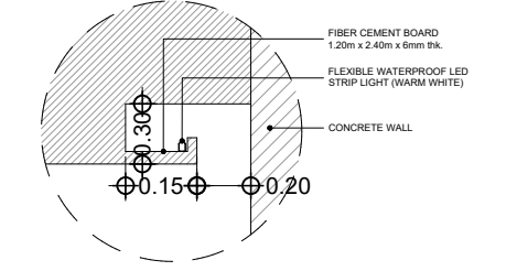
BLOW - UP DETAIL "D"
