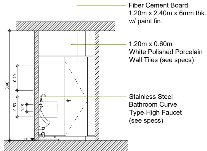
(COMMON C.R.) B SECTION - ELEVATION "A" A-08 SCALE 1:50M
