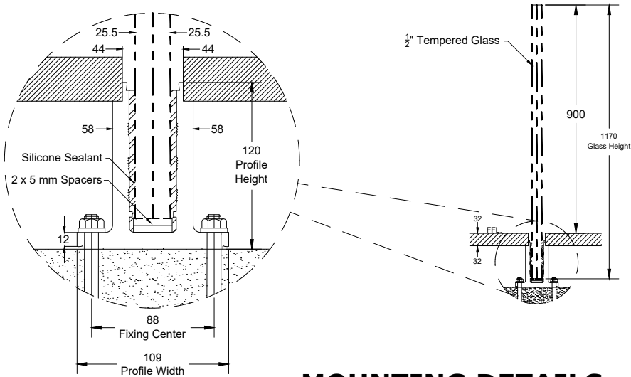
MOUNTING DETAILS
