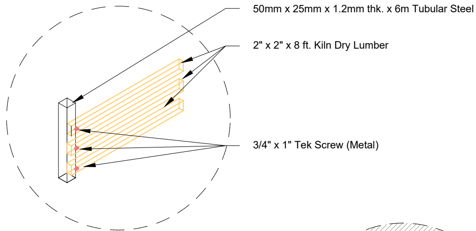
C A-13 SCALE NTS. SUNBREAKER BLOW-UP DETAIL "A"
