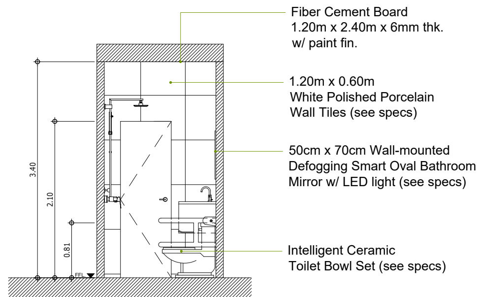
B (T&B - UNIT 101 & ROOM 101) A-07 SECTION - ELEVATION "A" SCALE 1:50M
