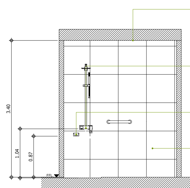
(T&B - UNIT 101 & ROOM 101) C SECTION - ELEVATION "B" A-07 SCALE 1:50M
