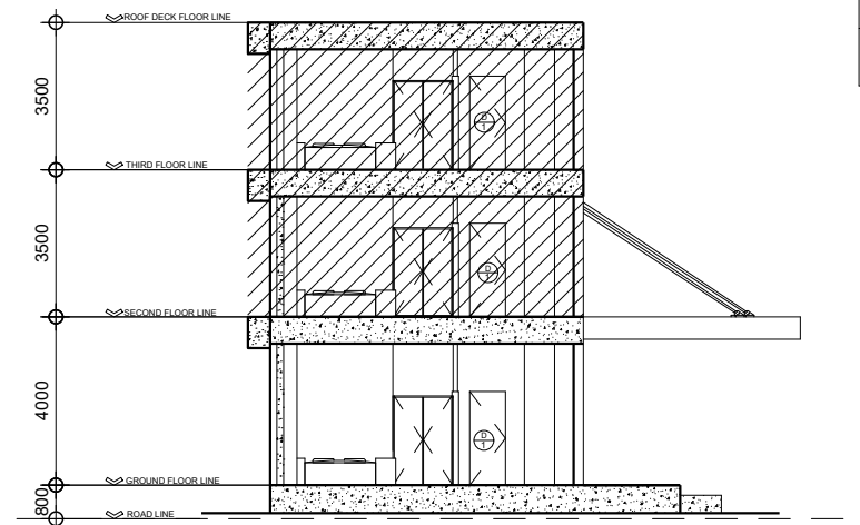
B CROSS SECTION A-04 SCALE 1:200M
