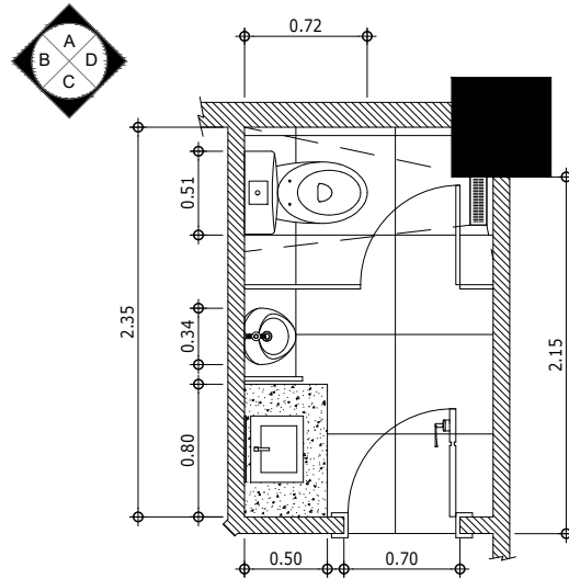
A PLAN (COMMON C.R.) A-08 SCALE 1:50M
