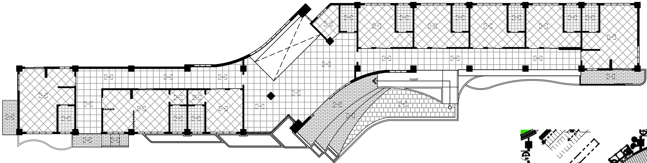
A TILES LAYOUT PLAN A-05 SCALE 1:200M
