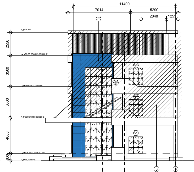
B RIGHT ELEVATION A-04 SCALE 1:200M
