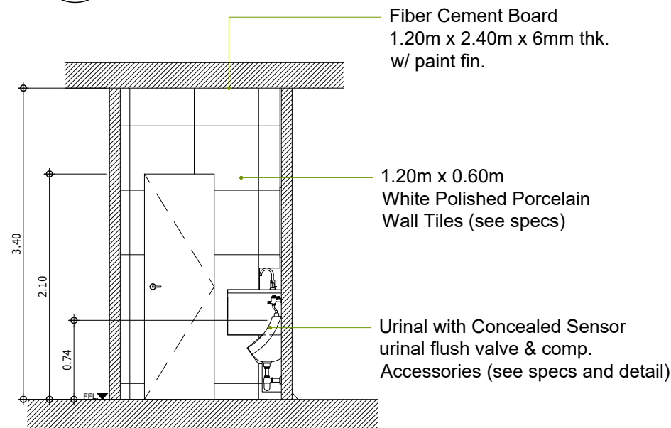
(COMMON C.R.) C SECTION - ELEVATION "B" A-08 SCALE 1:50M
