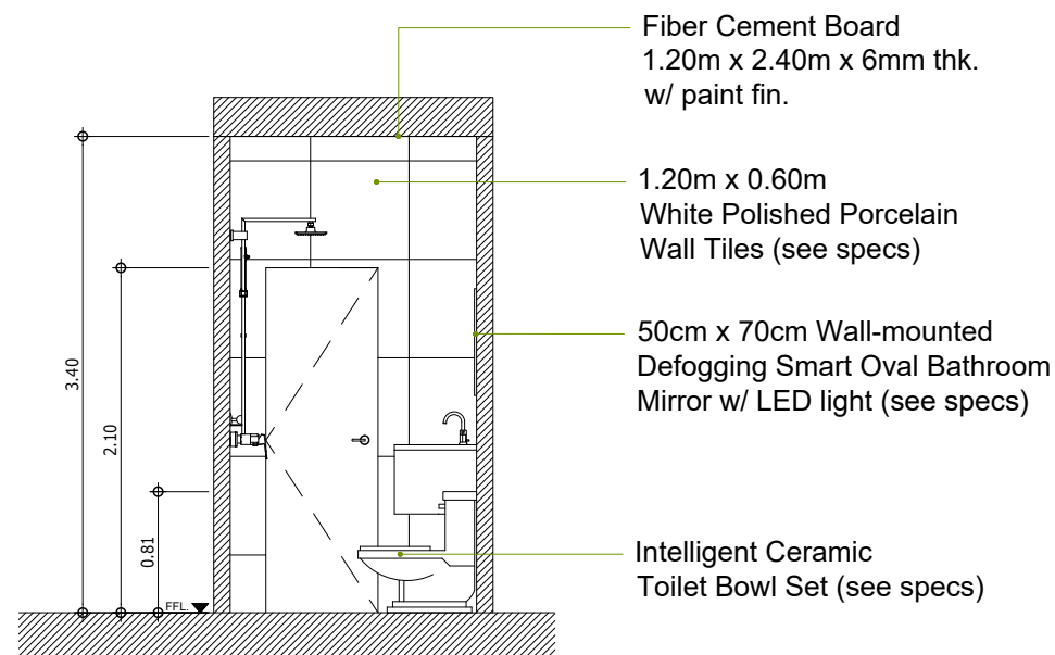
(T&B - UNIT 101 & ROOM 101) B SECTION - ELEVATION "A" A-07 SCALE 1:50M
